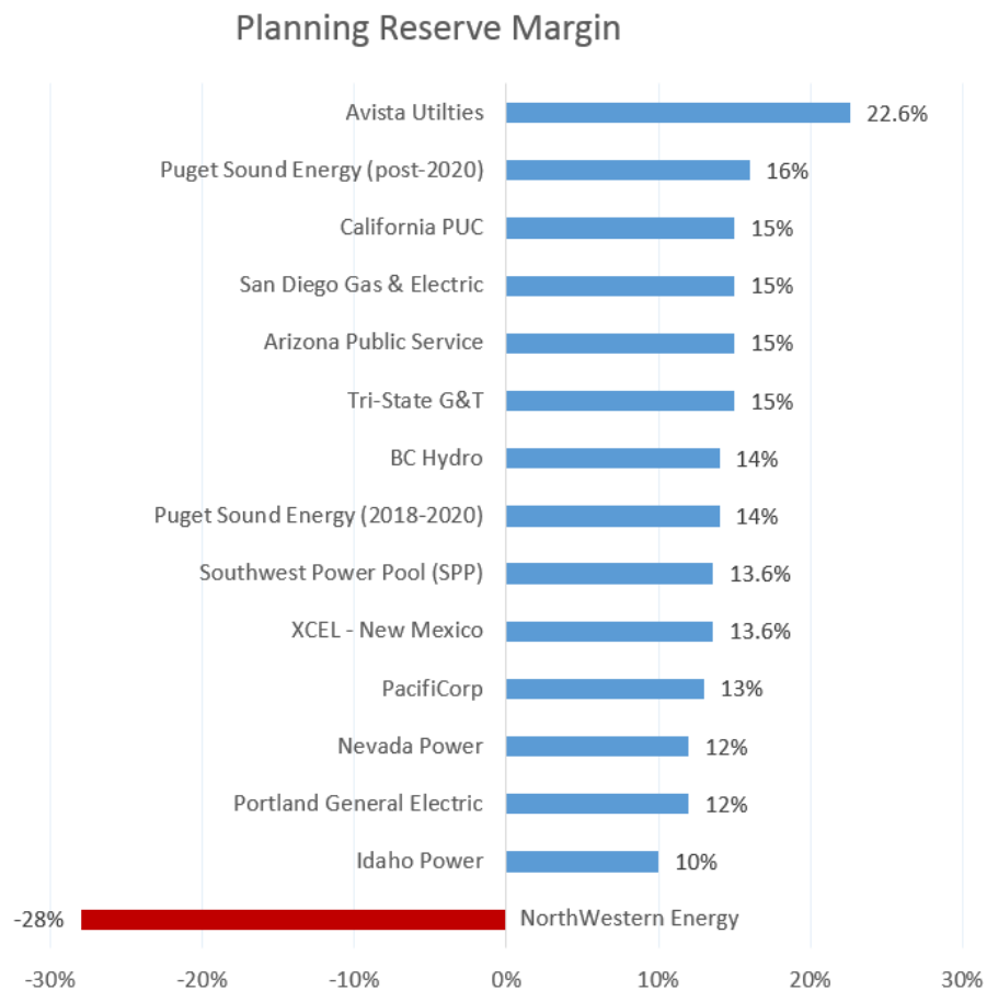
Figure 7-2 Planning Reserve Margins for Selected Power Companies
