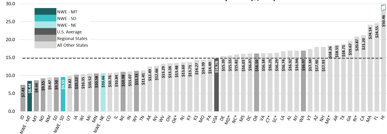
Residential Natural Gas Rates by State ($/Dkt)
